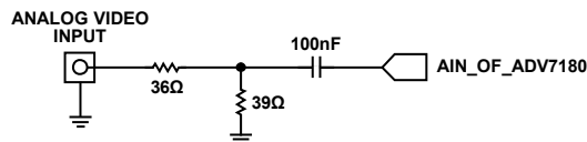
Figure 24. Input Voltage Divider Network
